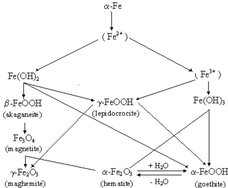
Figure 2 – Hiller scheme for the iron rust compounds [12].
